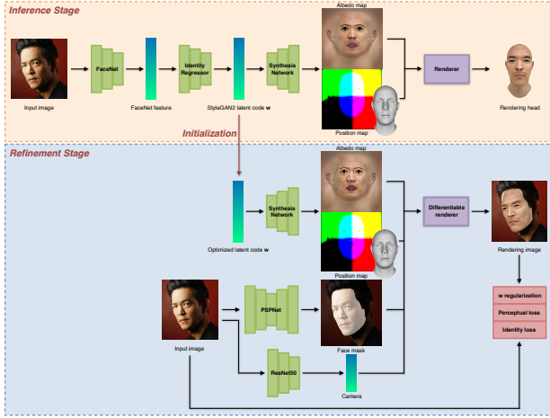
Figure 3: Two-stage facial digitization framework. The avatar is firstly predicted in the inference stage, and then improved to match the input image in the refinement stage.
