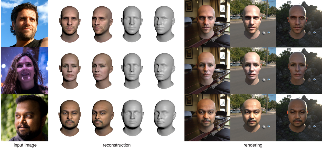
Figure 1: Given a single photograph, we can reconstruct a high-quality textured 3D face with neutral expression and normalized lighting condition. Our approach can handle extremely challenging cases and our generated avatars are animation friendly and suitable for complex relighting in virtual environments.
