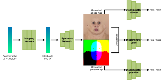
Figure 4: GAN-based geometry and texture synthesis.
